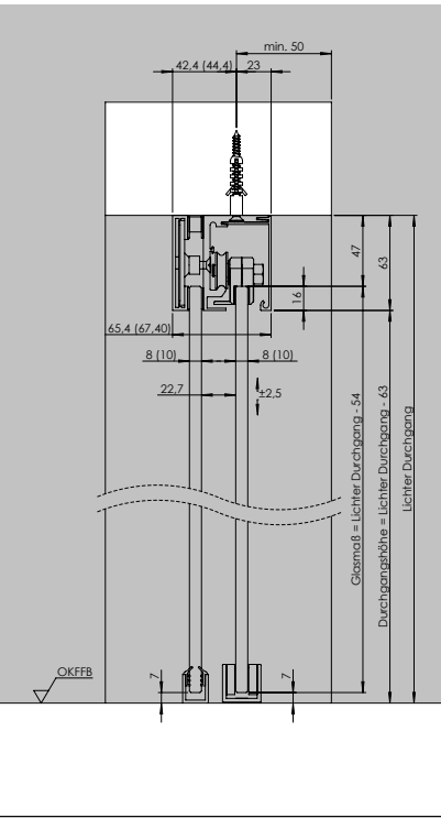
PLANEO 120, DECKENMONTAGE FÜR GLASANLAGEN CEILING MOUNTING FOR GLASS DOOR SYSTEM
